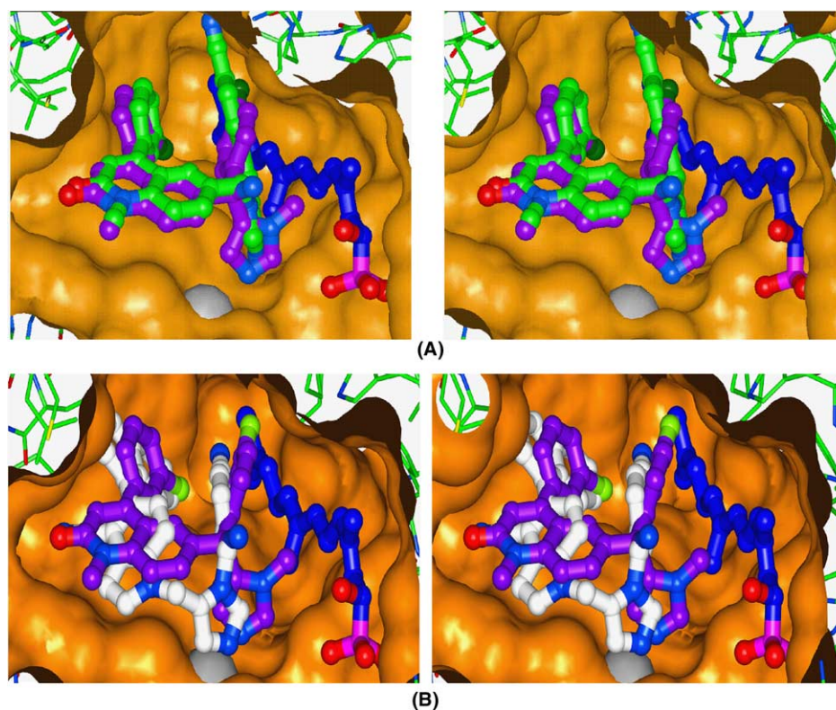
Figure 2. Stereoviews of overlays of models of (A) compound 3a (in green) and (B) compound 4d (in white) over the X-ray crystal structure of tipifarnib ( 1 ) 4 (in purple) in complex with FTase in the active site. Zn +2 is shown in grey and hydroxy farnesylpyrophosphate in blue.
