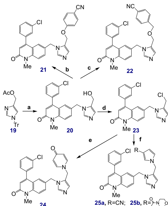
Scheme 4. Reagents and conditions: (a) (i) 11 , AcOEt, 60 °C, overnight; (ii) MeOH, reflux, 1 h; (iii) LiOH, THF/H 2 O, rt, 14 h, 57%; (b) 4-fluorobenzonitrile, NaH, DME, rt, overnight, 80%; (c) 4-cyanobenzyl bromide, NaH, DME, rt, 3 h, 40%; (d) SOCl 2 , rt, 1 h, 100%; (e) 4-hydroxypyridine, NaH, DME, rt, 14 h, 79%; (f) the pyrroles, 14 NaH, THF, rt, overnight, 36–37%.
