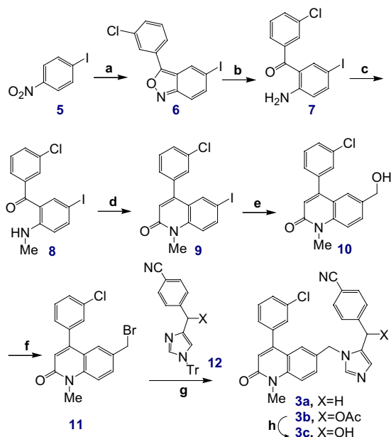
Scheme 1. Reagents and conditions: (a) 3-chlorophenylacetone, NaOH, MeOH, 0 °C to rt, 2 days, 93%; (b) Fe, AcOH, rt, 2 h, 49%; (c) Me 2 SO 4 , n -Bu 4 NBr, THF, 60 °C, 3.5 h, 86%; (d) (i) Ac 2 O, toluene, reflux, 21 h; (ii) NaOH, EtOH/H 2 O, reflux, 1.5 h, 96%; (e) (i) iso -PrMgBr, THF, –25 °C, 50 min, then N -formylmorpholine, rt, overnight, 80%; (ii) NaBH 4 , MeOH, –78 °C to rt, overnight, 87%; (f) PBr 3 , LiBr, DMF 0 °C to rt, 2 h, 96%; (g) (i) AcOEt, 55 °C, 4 days; (ii) MeOH, reflux, 2 h, 42–46%; (h) LiOH, THF/H 2 O, rt, overnight, 100%.
