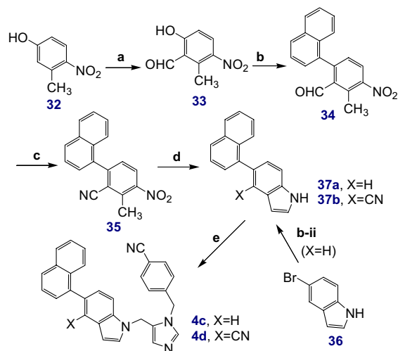
Scheme 6. Reagents and conditions: (a) hexamethylenetetramine, TFA, reflux, 60 h, 8%; (b) (i) Tf 2 O, Et 3 N, CH 2 Cl 2 , rt, overnight, 87%; (ii) 1-naphthylboronic acid, Pd(PPh 3 ) 4 , NaHCO 3 , EtOH/toluene, reflux, 3 h, 37–46%; (c) (i) NH 2 OH, NaOAc, EtOH, reflux, overnight; (ii) Ac 2 O, reflux, 4 h, 93%; (d) (i) DMF–DMA, DMF, 100 °C, 3 h; (ii) Fe, AcOH/EtOH, reflux, 0.5 h, 59%; (e) 31a , NaH, DMF, rt, overnight, 20–22%.
