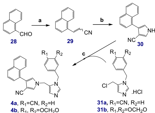
Scheme 5. Reagents and conditions: (a) CNCH 2 PO(OEt) 2 , DBU, CH 3 CN, rt, overnight, 100%; (b) TosMIC, t -KOBu, THF, reflux, 2 h, 75%; (c) NaH, THF, rt, 5 h, 75–88%.
