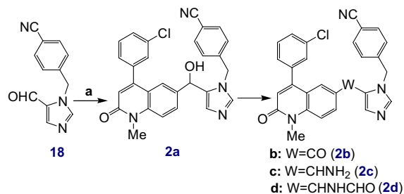
Scheme 3. Reagents and conditions: (a) iso -PrMgBr, THF, –25 °C, 30 min, then 18 , rt, overnight, 38%; (b) MnO 2 , dioxane, reflux, 1 h, 80%; (c) (i) SOCl 2 , CH 2 Cl 2 , rt, 2 h; (ii) NH 4 OH, THF/H 2 O, rt, 1 h, 32%; (d) HCONH 2 , AcOH, reflux, 5 h, 100%.
