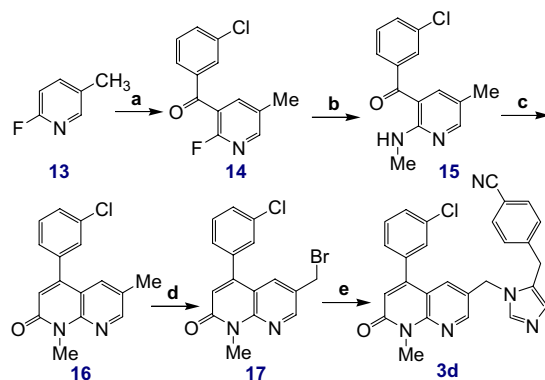
Scheme 2. Reagents and conditions: (a) (i) LDA, THF, –78 °C, 2 h, then 3-chlorobenzaldehyde, rt, overnight, 66%; (ii) MnO 2 , dioxane, reflux, 1 h, 94%; (b) MeNH 2 , EtOH, rt, 5 h, 93%; (c) (i) AcOBu t , LDA, THF, –78 °C to rt, overnight; (ii) toluene, reflux, 1 h, 84%; (d) NBS, AIBN, CCl 4 , reflux, 5 h, 44%; (e) 12 , AcOEt, 55 °C, 5 days, then MeOH, reflux, 2 h, 55%.
