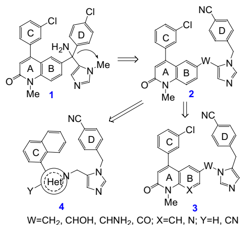
Figure 1. Modifications of tipifarnib ( 1 ) lead to novel inhibitors of FTase 2 , 3 , and 4 .
